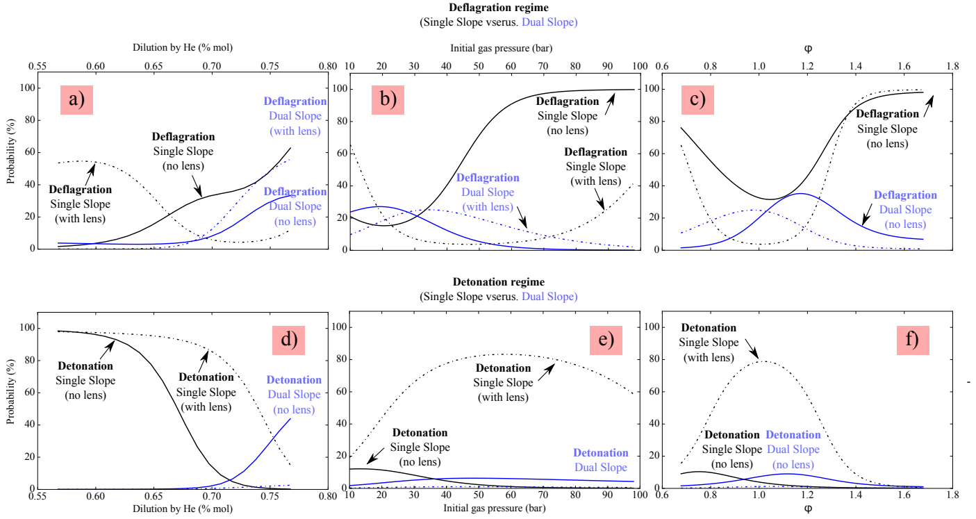
Figure 3: Deflagration regime probability considering both ignition sources and single/dual slope phenomenon in average conditions, regarding a) dilution by He, b) initial gas pressure and c) equivalence ratio. Detonation regime probability considering both ignition sources and single/dual slope phenomenon in average conditions, regarding d) dilution by He, e) initial gas pressure and f) equivalence ratio.
