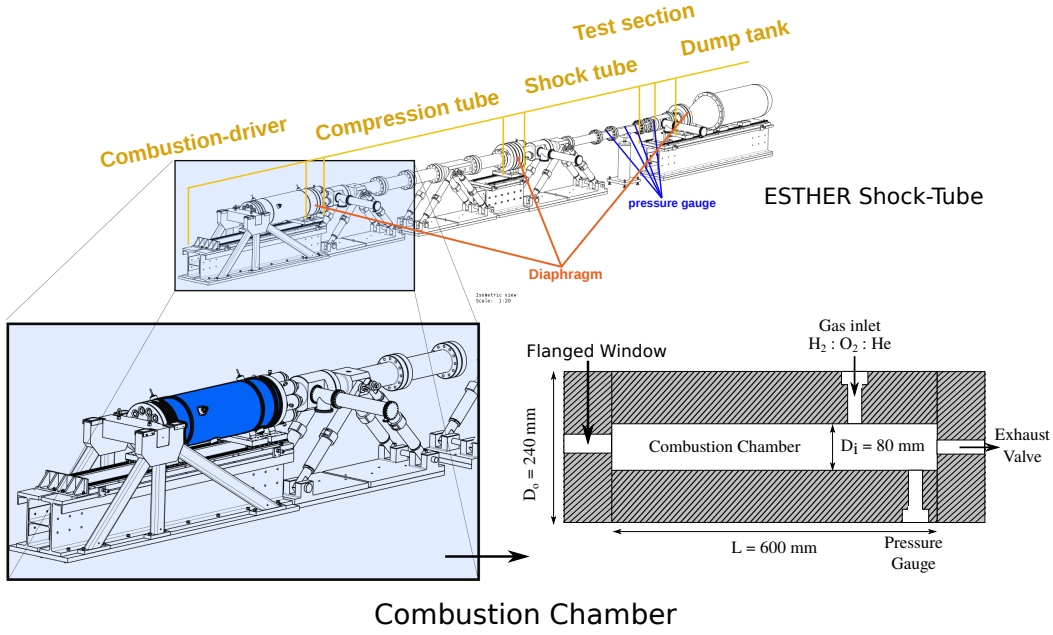
Figure 1: Schematic representation of the closed combustion chamber.
